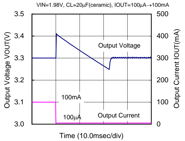
XC9104D093MR(PWM/PFM,300kHz,3.3V)
