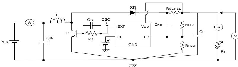
CIRCUIT ③
