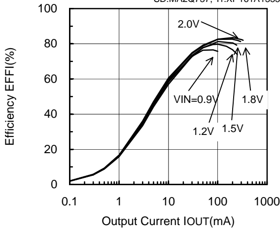
XC9103D092MR (PWM,180kHz,3.3V)
