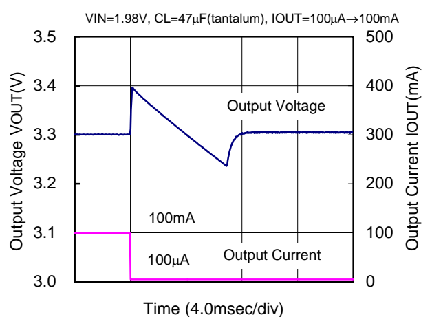
XC9104D092MR(PWM/PFM,180kHz,3.3V)
