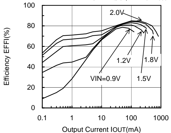
XC9104D093MR (PWM/PFM,300kHz,3.3V)
