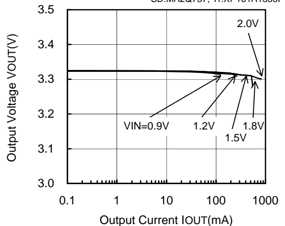
XC9104D093MR (PWM/PFM,300kHz,3.3V)
