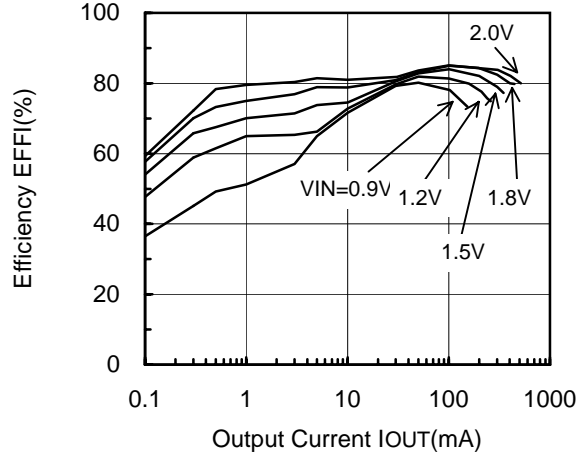
XC9104D092MR (PWM/PFM,180kHz,3.3V)
