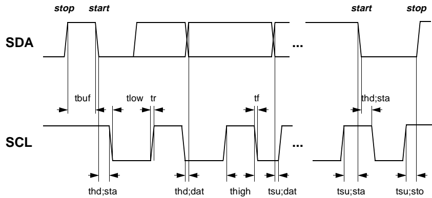
Figure 6.11 : Serial Interface Timing Characteristics
