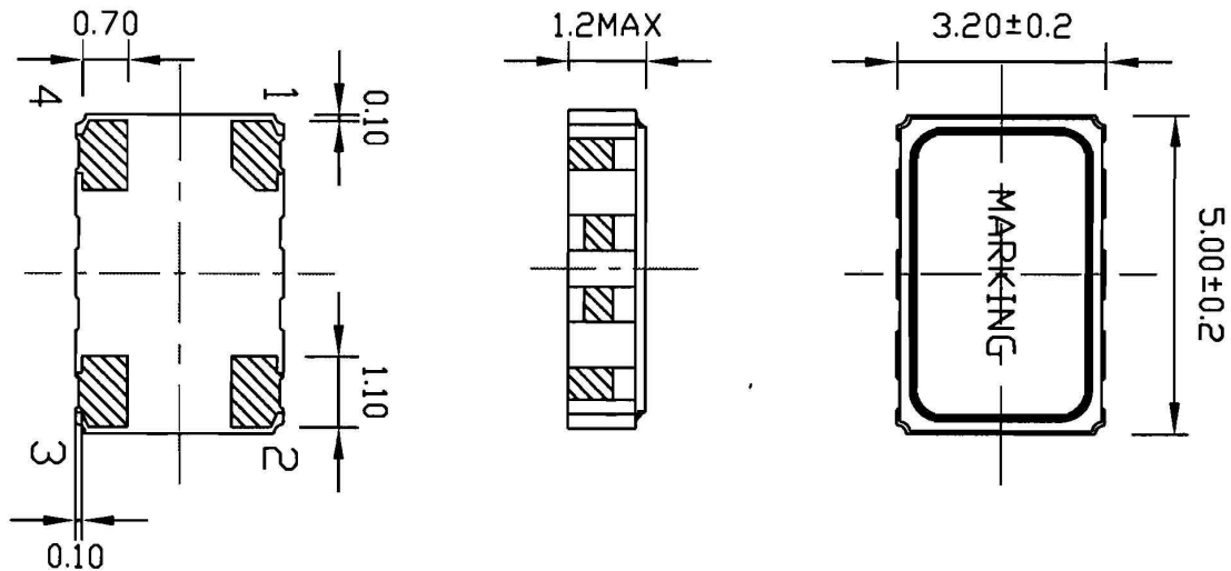
Contact Pads are gold over nickel Devices will be marked with the frequency Figure 3, Package drawing
