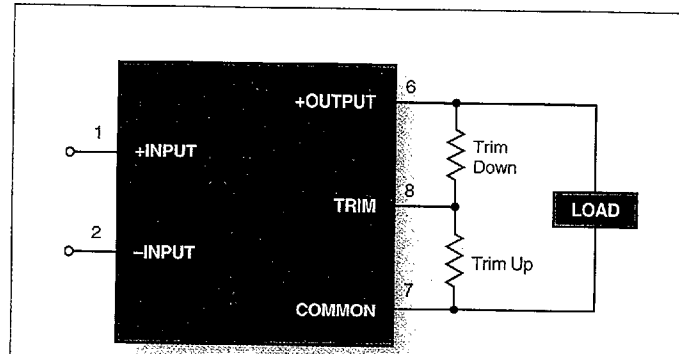
Figure 2a. Trim Connections Using a Trimpot
