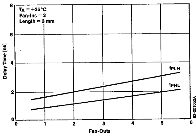
Delay Time vs Fan-Outs [NAND]
