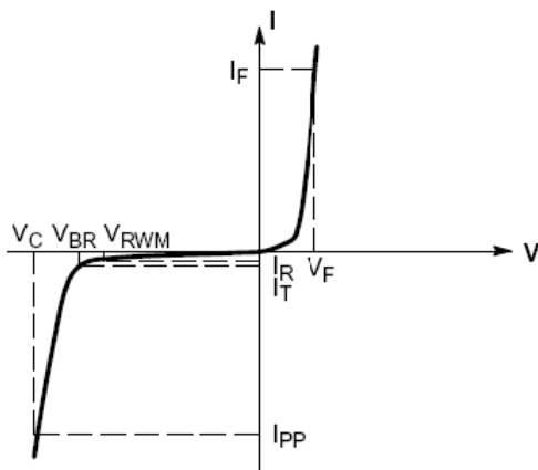
Uni-Directional TVS
