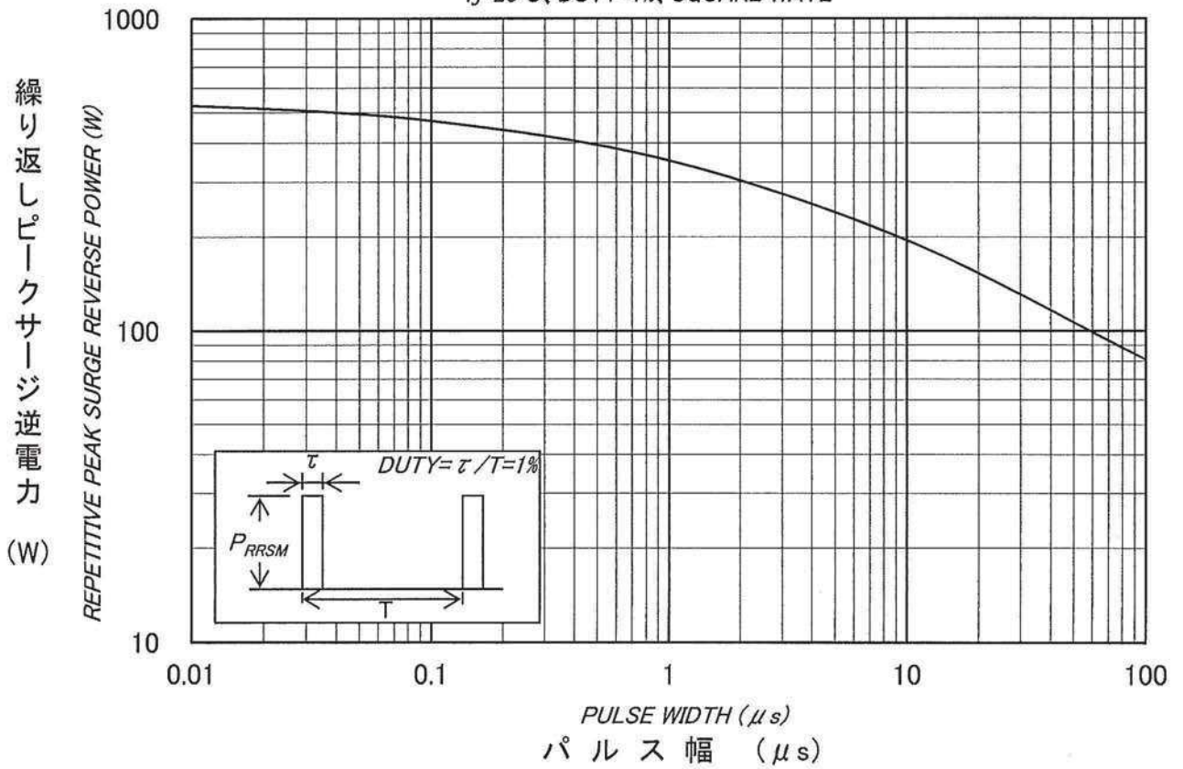
繰り返しピークサージ逆電力定格 REPETITIVE PEAK SURGE REVERSE POWER RATINGS T_j=25^\circ\text{C} , DUTY=1%, SQUARE WAVE
