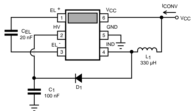
FIGURE 1: TYPICAL APPLICATION
