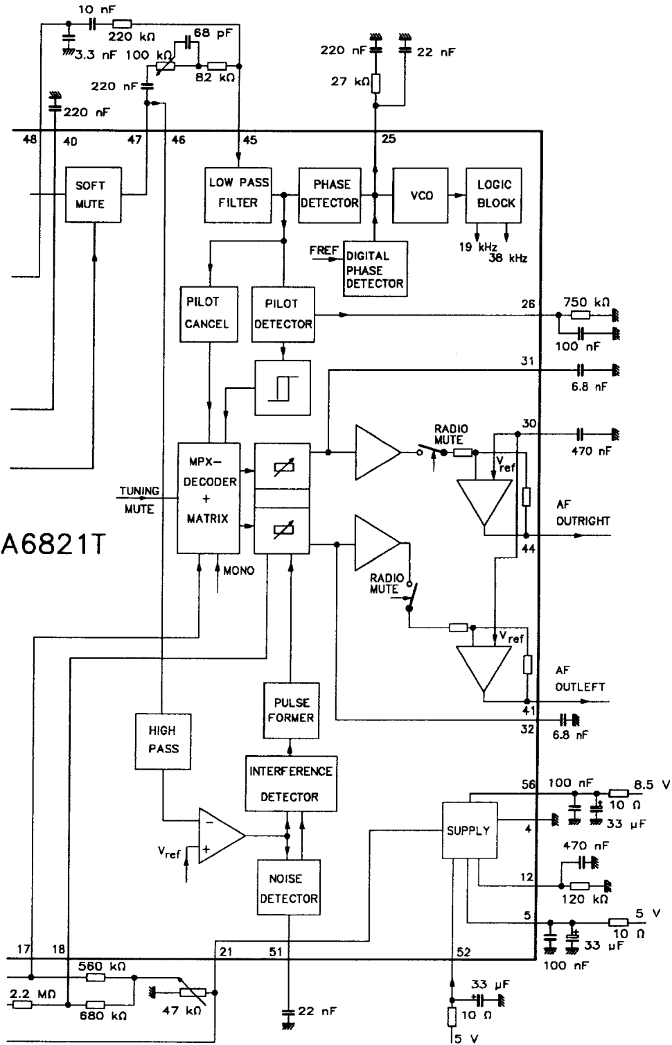
Fig.2 Block diagram (continued from Fig.1).
