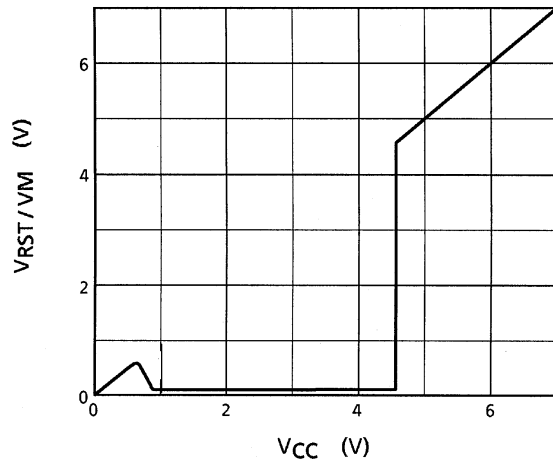
RESET/M OUTPUT CHARACTERISTIC
