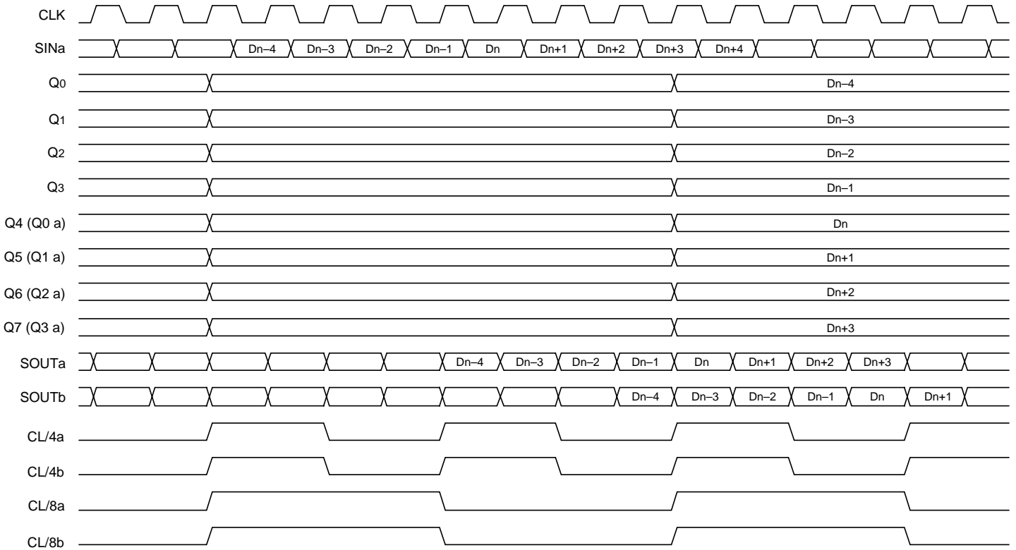
Timing Diagram
