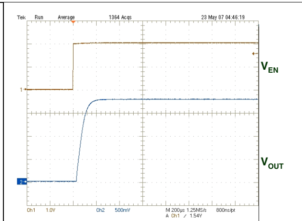
Figure 25. Enable transient
