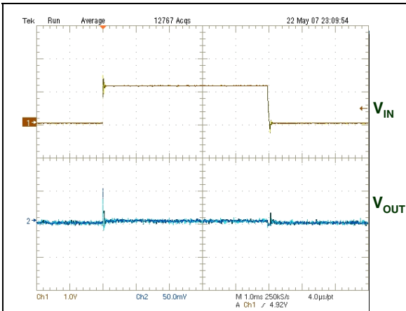
Figure 22. Line transient
