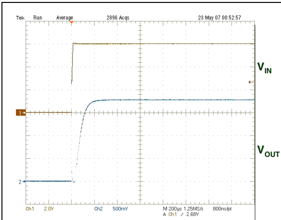
Figure 24. Start-up transient
