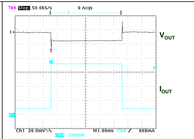
Figure 23. Load transient
