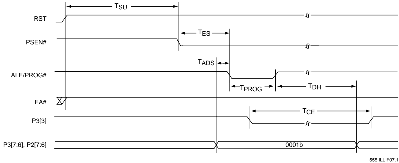
FIGURE 4-4: CHIP-ERASE
