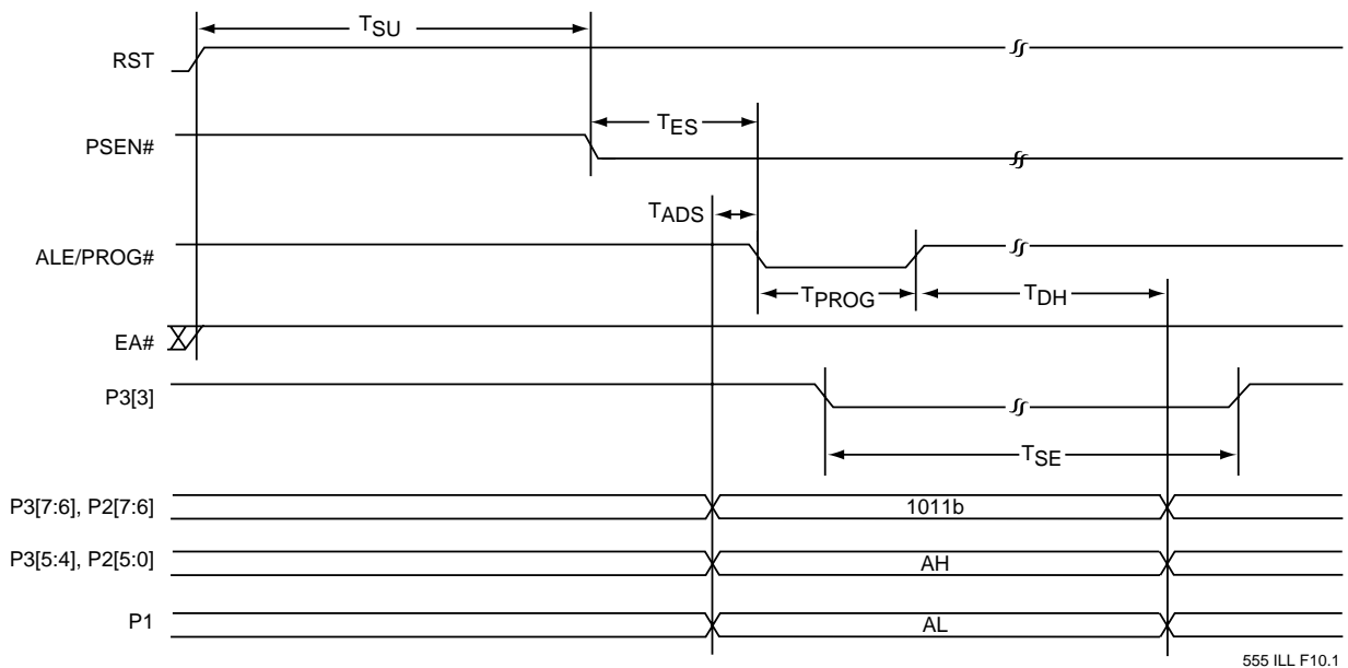
FIGURE 4-7: SECTOR-ERASE
