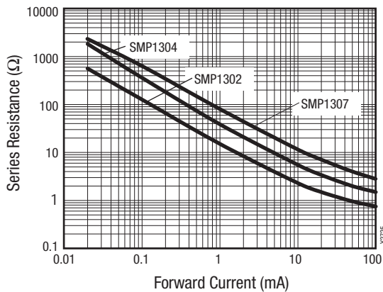
Figure 3. Series Resistance vs Forward Current @ 100 MHz
