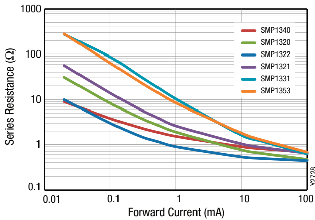
Figure 1. Series Resistance vs Forward Current @ 100 MHz
