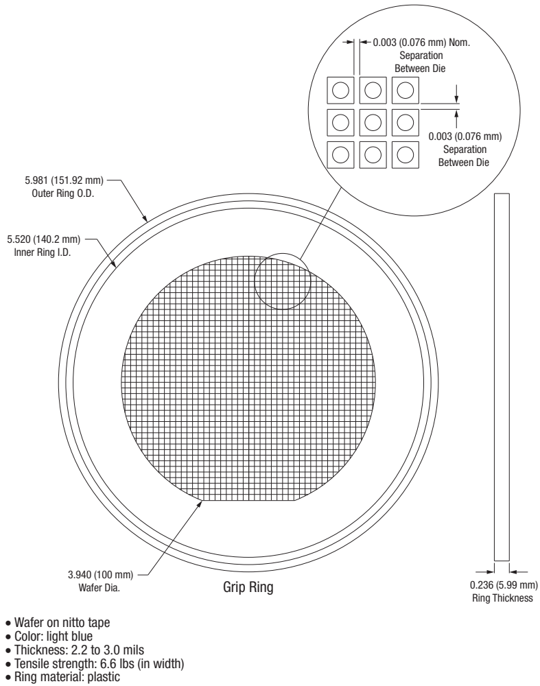
Figure 5. Wafer Film Frame Description
