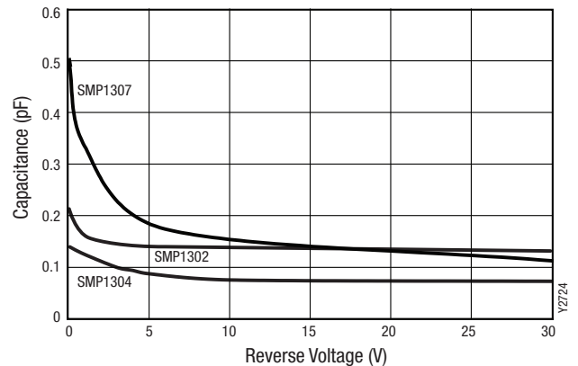
Figure 4. Capacitance vs Reverse Voltage
