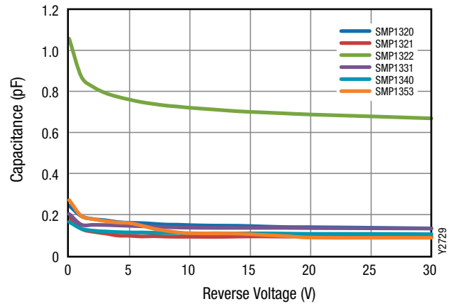
Figure 2. Capacitance vs Reverse Voltage
