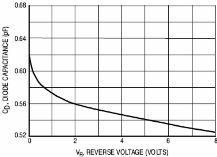
Figure 3. Capacitance
