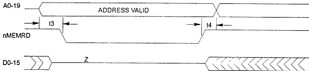
FIGURE 28 - 8-BIT MODE REGISTER CYCLES
