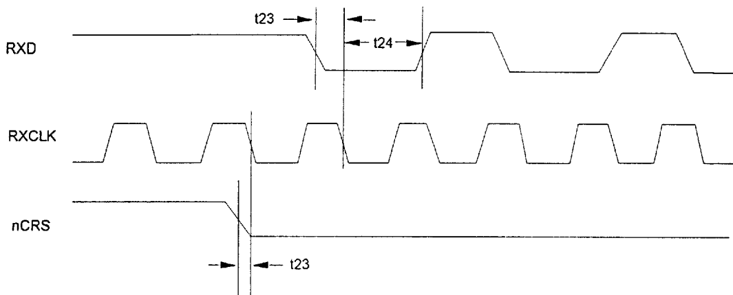
FIGURE 35 - EXTERNAL ENDEC INTERFACE - START OF TRANSMIT
