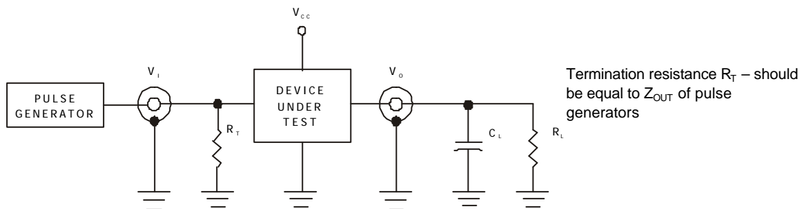
Figure 2. Test Circuit
