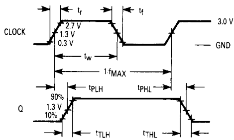
Figure 1. Switching Waveforms
