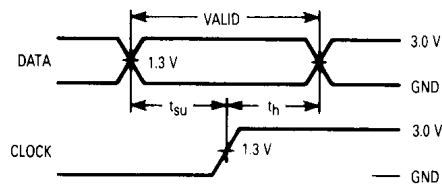
Figure 3. Switching Waveforms
