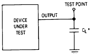
Figure 3. Test Circuit
