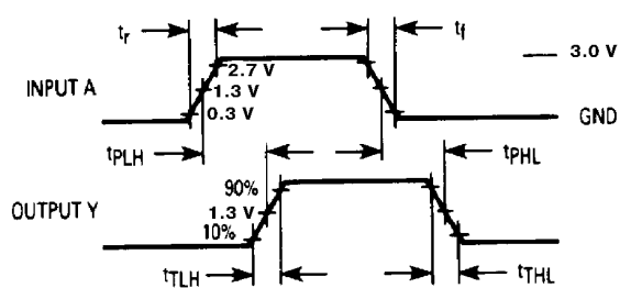
Figure 1. Switching Waveforms
