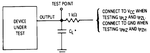
Figure 4. Test Circuit
