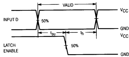
Figure 4. Switching Waveforms
