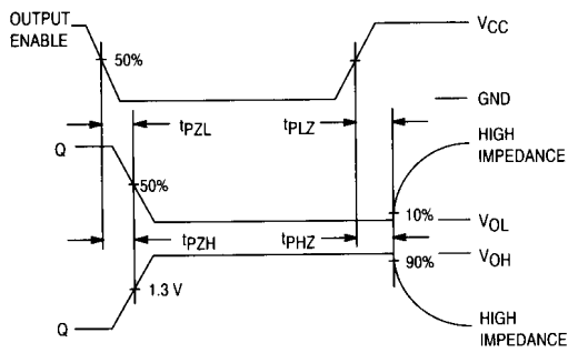
Figure 3. Switching Waveforms
