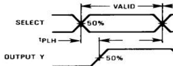
Figure 2. Switching Waveforms
