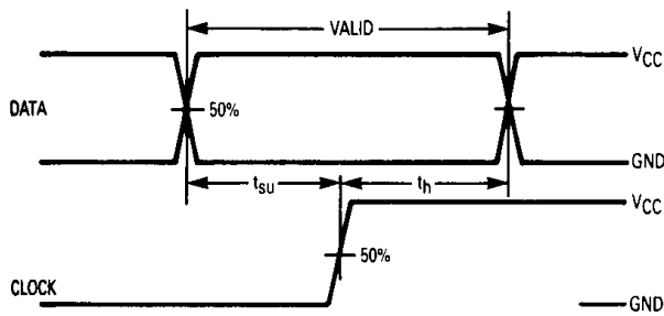
Figure 3. Switching Waveforms
