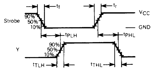
Figure 4. Switching Waveforms
