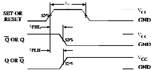
Figure 2. Switching Waveforms
