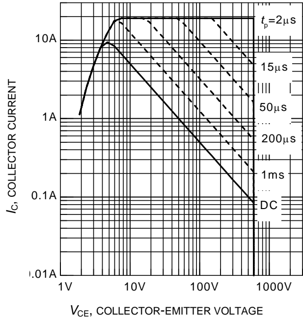
Figure 2. Safe operating area ( D = 0 , T_C = 25^\circ\text{C} , T_i \leq 150^\circ\text{C} )
