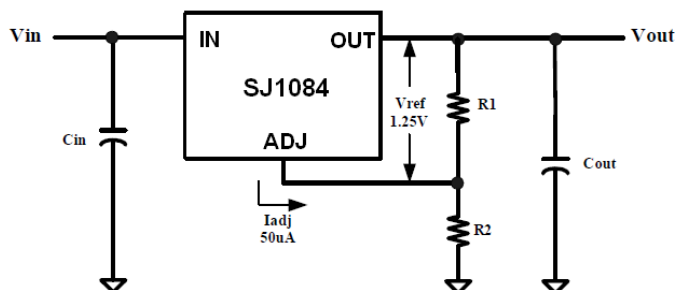
Figure1. Adjustable Voltage Regulator
