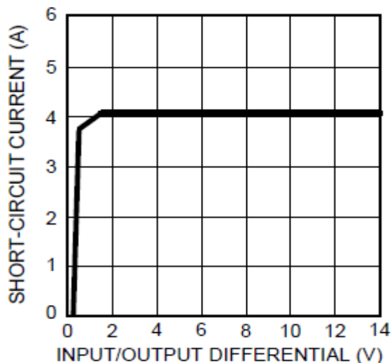
Short-Circuit Current
