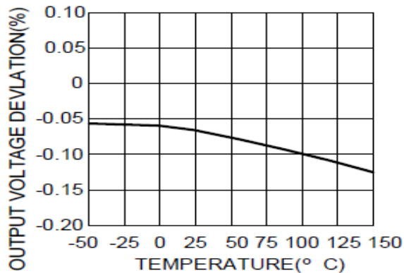
Load Regulation
