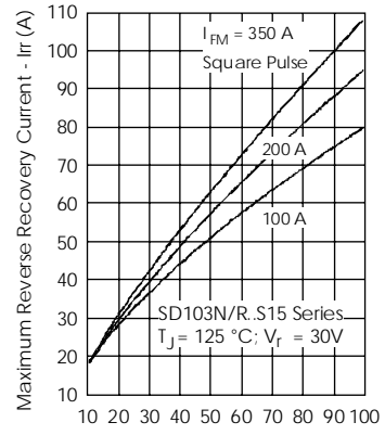
Fig. 15 - Recovery Current Characteristics
