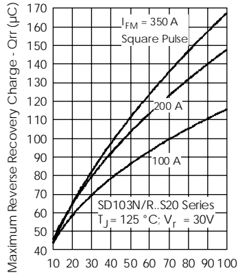
Fig. 17 - Recovery Charge Characteristics
