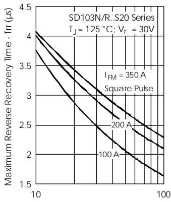
Fig. 16 - Recovery Time Characteristics
