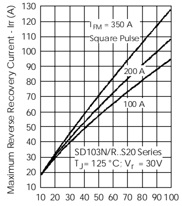
Fig. 18 - Recovery Current Characteristics
