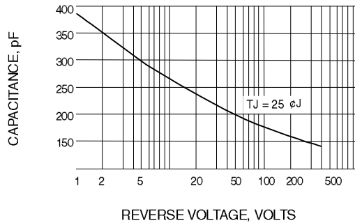
Fig. 5-TYPICAL JUNCTION CAPACITANCE
