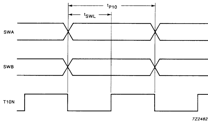
Fig.4 Data input timing (pins 59, 61 and 63).
