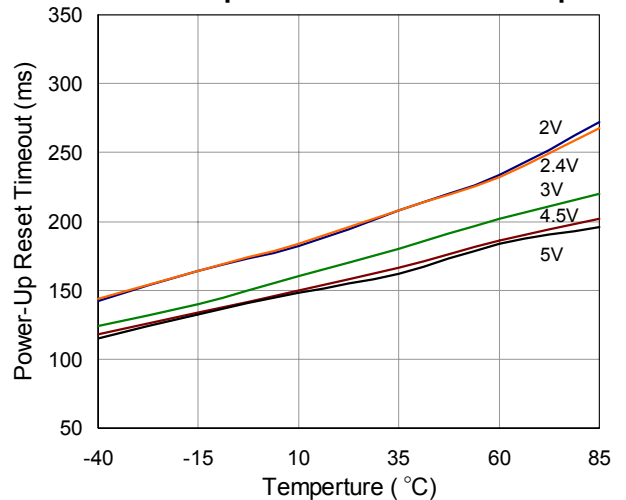
Power-Up reset Timeout vs. Temp.
