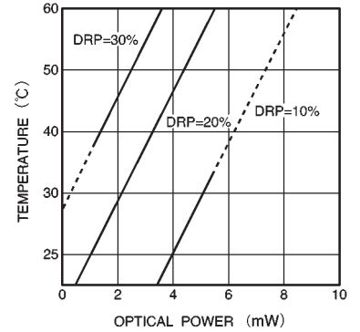
Fig. 9 Temperature vs. output guidelines for various droop percentages
