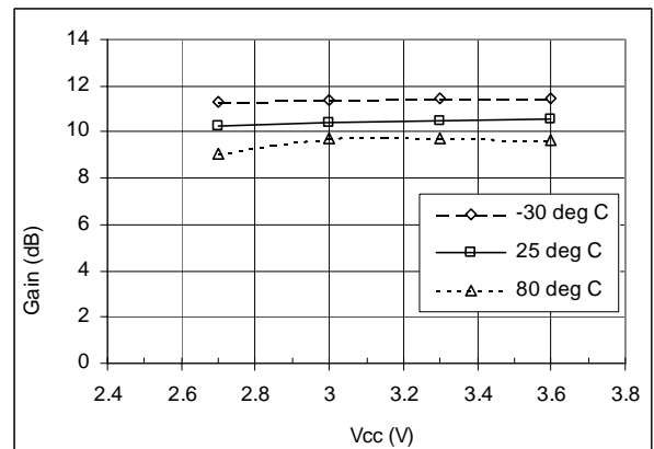
Figure 12. PCS Mixer Conversion Gain (RF Frequency = 1960 MHz, LO Frequency = 1749.62 MHz, IF Frequency = 210.38 MHz)
