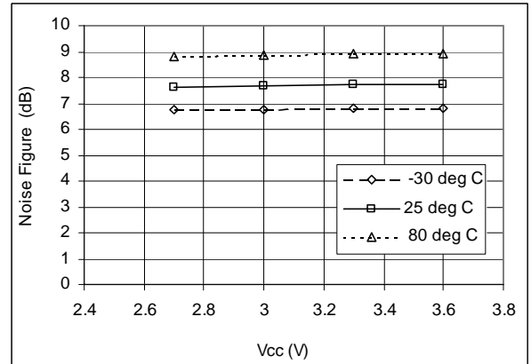
Figure 10. CDMA Mixer Noise Figure (RF Frequency = 881.52 MHz, LO Frequency = 966.90 MHz, IF Frequency = 85.38 MHz)
