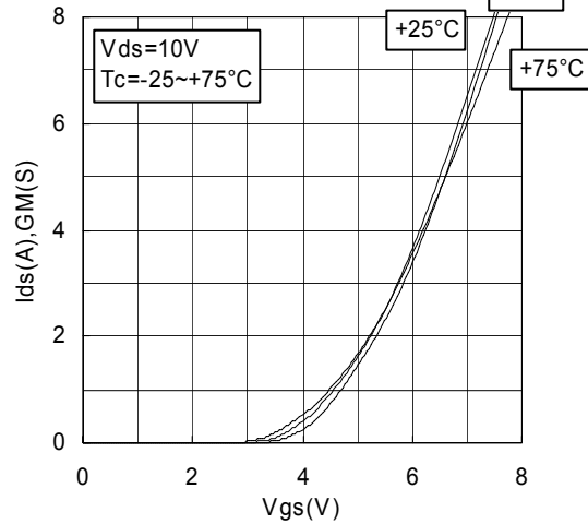
Vgs-Ids CHARACTERISTICS 2
