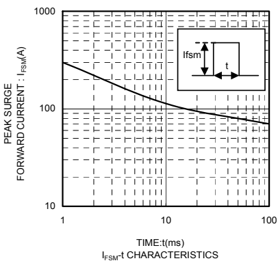
I_{FSM} - t CHARACTERISTICS
