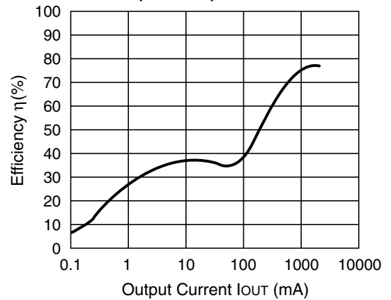
R1225N182D (V IN =12V) CDRH127-10uH
