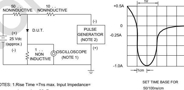
FIG.4-TEST CIRCUIT DIAGRAM AND REVERSE RECOVERY TIME CHARACTERISTIC
