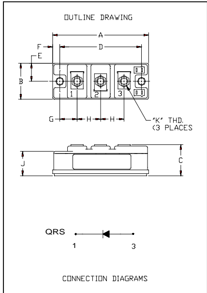
QRS1440T30 Fast Recovery Diode Module 400 Amperes / 1400 Volts
