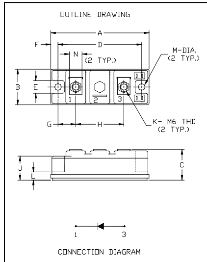
QRS0640T30 Fast Recovery Diode Module
