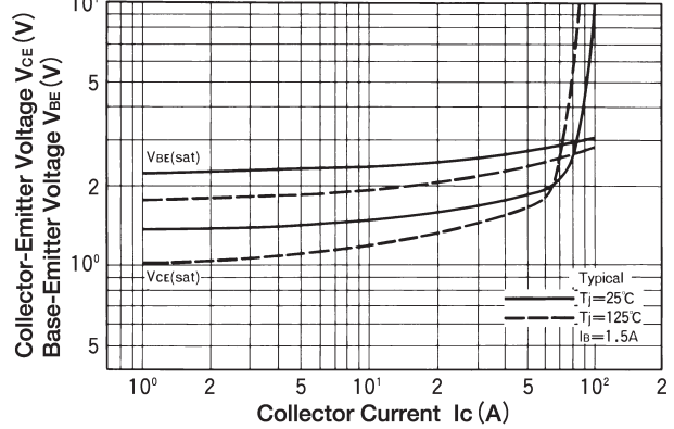
Saturation Characteristics
