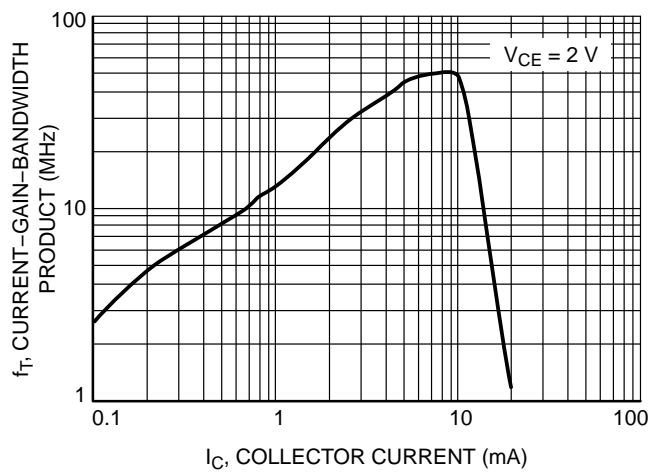
Figure 6. Current-Gain-Bandwidth Product
