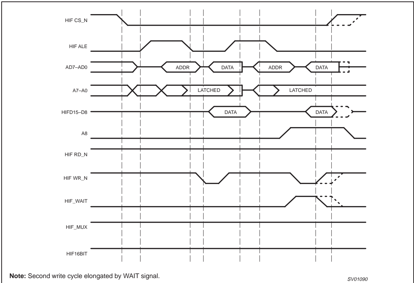
Figure 8. 16 Bit Write Cycle Multiplexed
