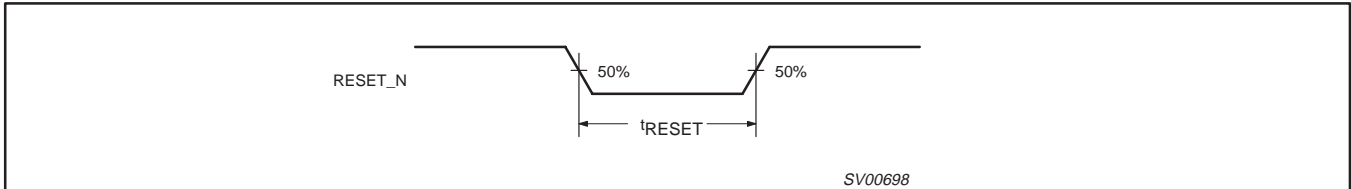
Figure 43. RESET_N Waveform
