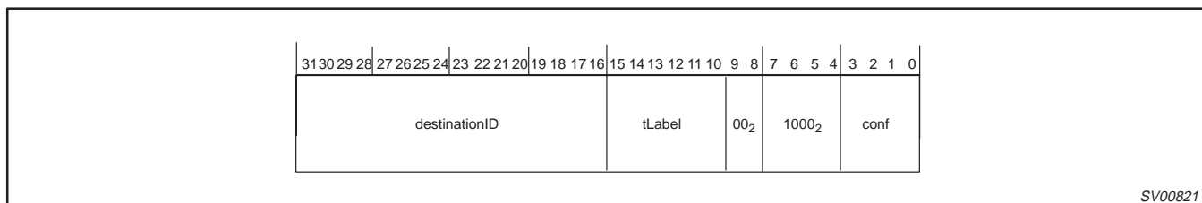
Figure 21. Request and response confirmation format
