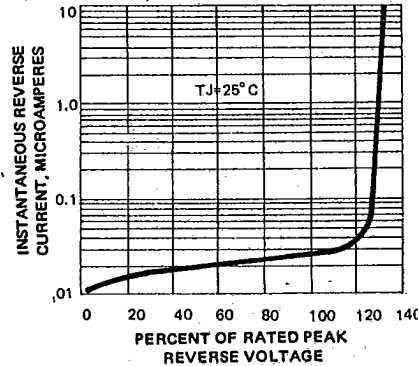
FIG. 4-TYPICAL REVERSE CHARACTERISTICS
