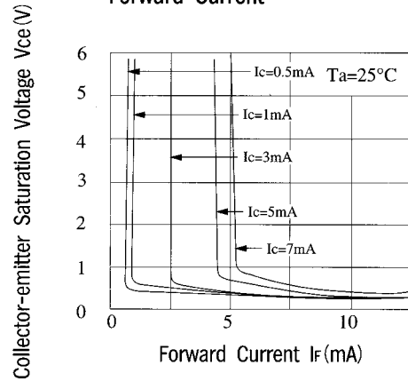
Fig. 9 Collector-emitter Saturation Voltage vs. Forward Current
