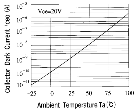
Fig. 3 Collector Dark Current vs. Ambient Temperature
