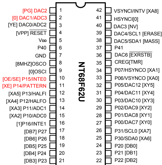
42-Pin S-DIP
