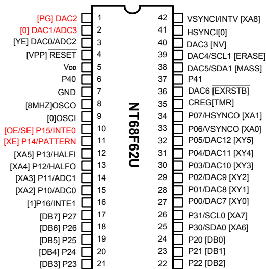
42-Pin S-DIP
