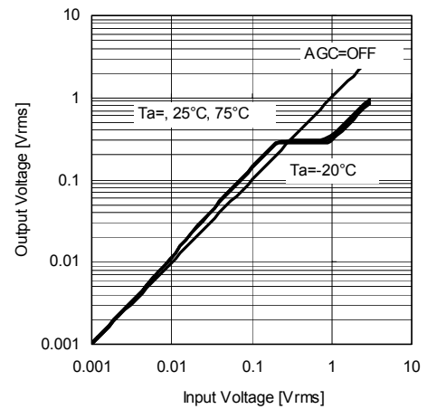
AGC Output Voltage vs. Input Voltage V+=9V, R L =47kΩ, Vin(A+Bch), f=1kHz, Vout(Ach), BW=400Hz-30kHz, VOL=0dB, BAL=0dB, AGC=300mV, BASS=TREB=0dB, BBE=OFF, Surround=OFF
