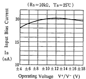
Input Bias Current vs. Operating Voltage ( R_s = 10k\Omega , T_a = 25^\circ C )
