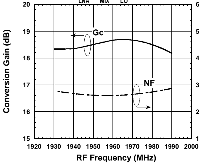
Conversion Gain , Noise Figure vs. RF Frequency ( V_{LNA}=V_{MIX}=V_{LO}=3.0\text{V} )
