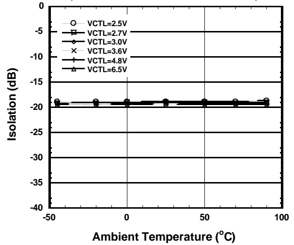
PC-P2 Isolation vs. Ambient Temperature ( PC-P3 ON ,f=1.9GHz ,Pin=32dBm )
