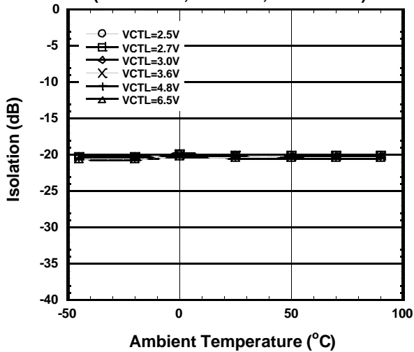
PC-P3 Isolation vs. Ambient Temperature ( PC-P4 ON ,f=1.9GHz ,Pin=32dBm )
