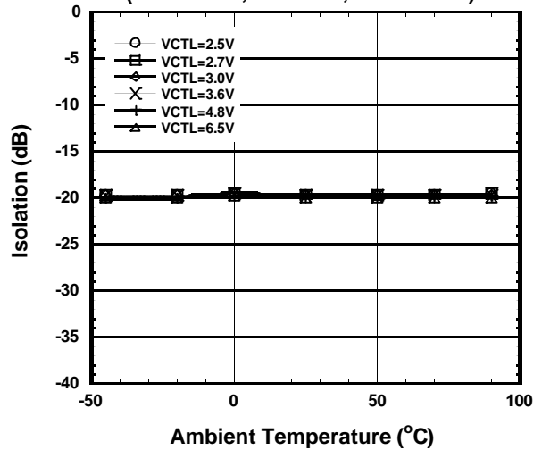
PC-P4 Isolation vs. Ambient Temperature ( PC-P1 ON ,f=1.9GHz ,Pin=32dBm )
