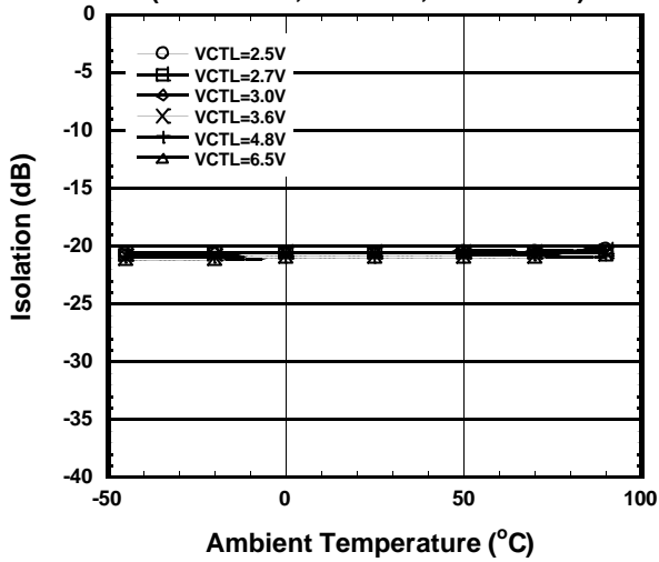
PC-P1 Isolation vs. Ambient Temperature ( PC-P2 ON ,f=1.9GHz ,Pin=32dBm )
